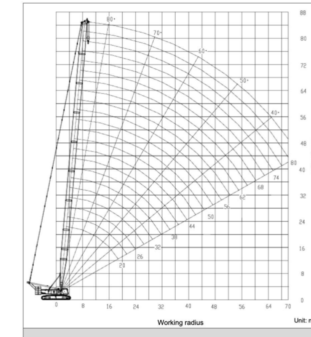
Characteristic curve of lifting height of operating mode S
